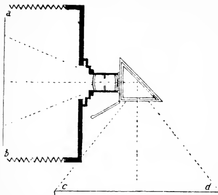
FIG. 31. Illustrating position of prism in plan— a b sensitive plate, c d copying-board.
